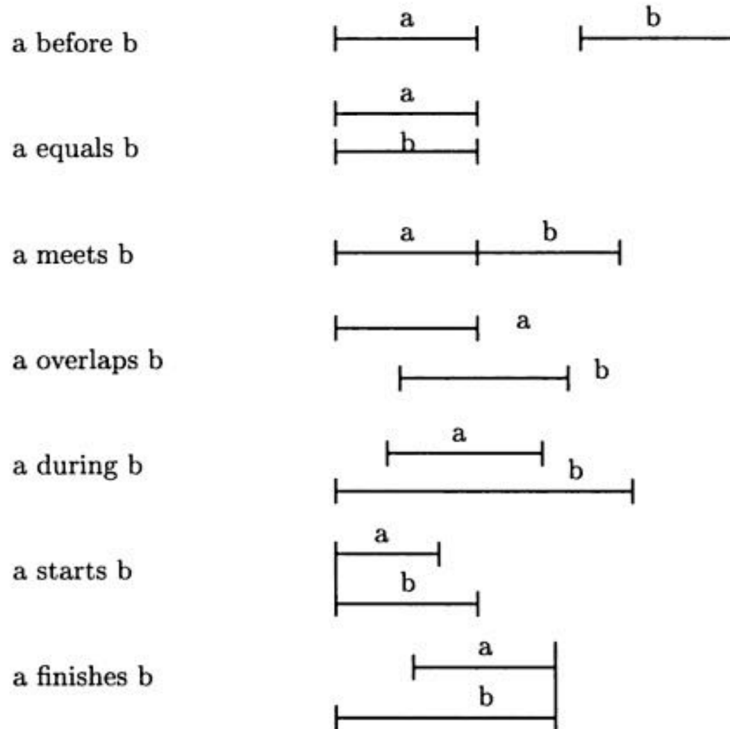
Figure 13.1 Allen's interval comparison operators
